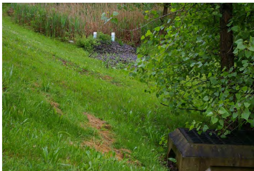
Figure 4. Grassed filter strip to infiltration basin.
